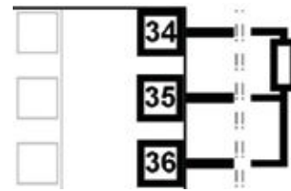
Figure 15. Input 2 - RTD Connections
