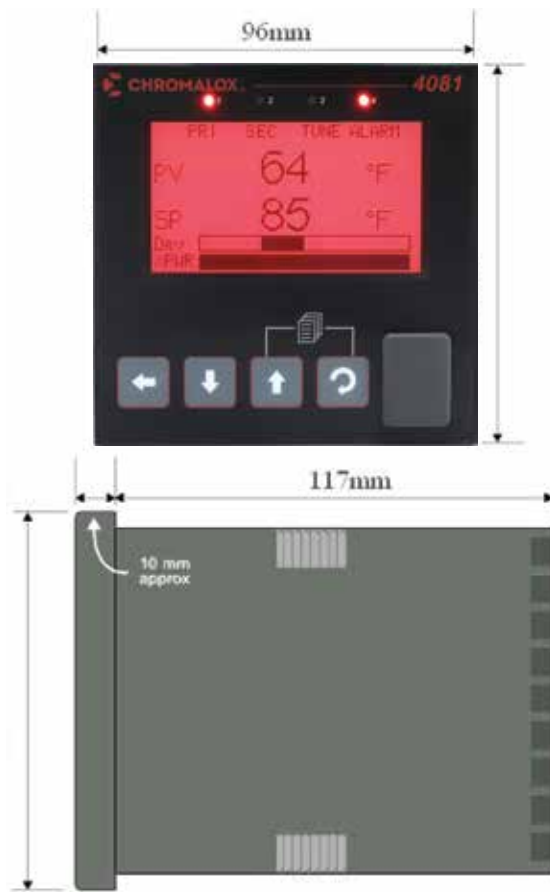
Figure 1. Main Dimensions
