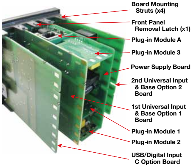
Figure 3. Rear View (uncased) & Board Positions
