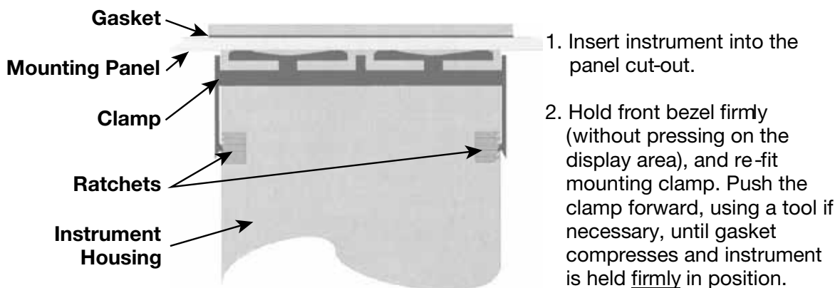
Figure 2. Panel-Mounting
