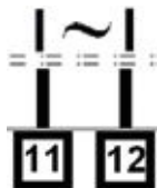
Figure 36. Plug-in Module Slot 3 - Triac Module
