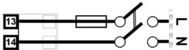
Figure 9. Mains Power Connections
