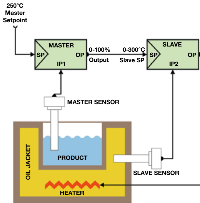
Figure 47. Cascade Example
