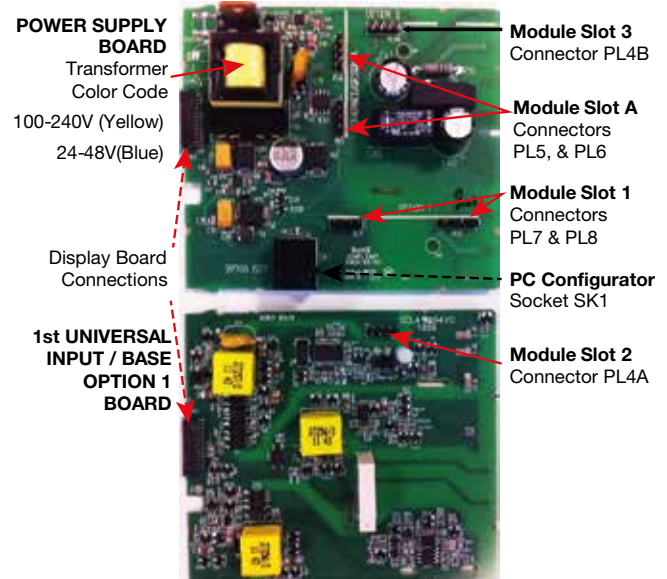
Figure 4. Main Board Connectors
