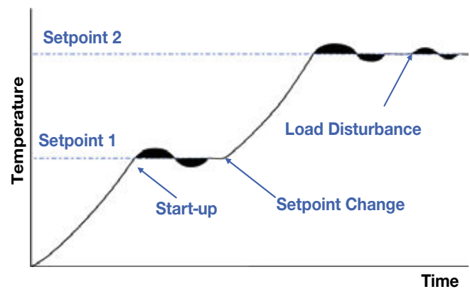
Figure 59. Self-Tune Operation
