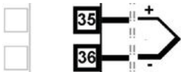
Figure 14. Input 2 - Thermocouple Connections
